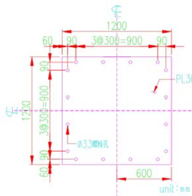
(a) 試體下部端板尺寸
