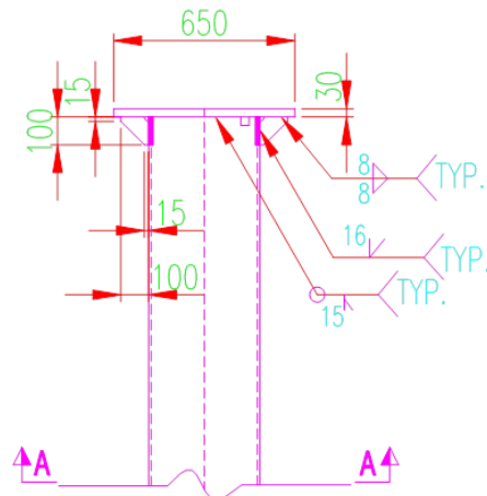
(b) 試體上部端板加勁
