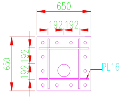
(c) 試體上部加勁板
