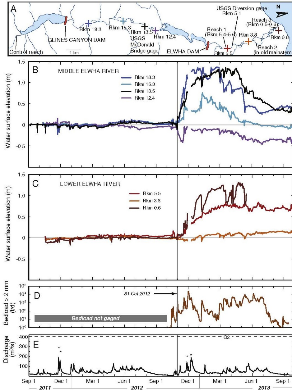
圖 3-7 Elwha River 水文泥砂監測 (East et al., 2014)
