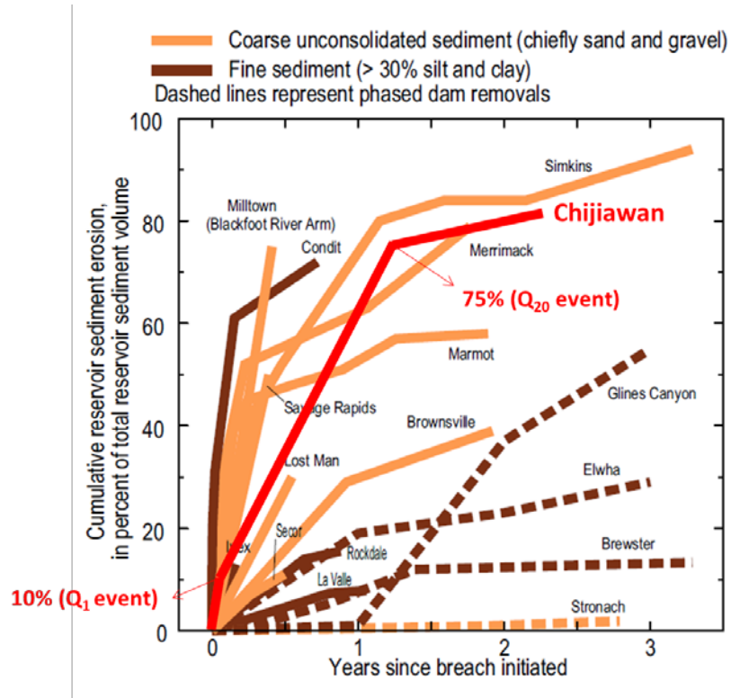
圖 3-19 不同泥砂組成與侵蝕土方量之關係(修改自 Sawaske and Freyburg, 2012; Grant and Lewis, 2015; Major et al., 2017)
