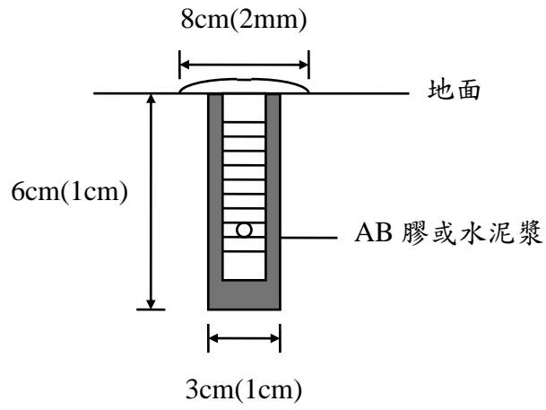
(側視圖)
